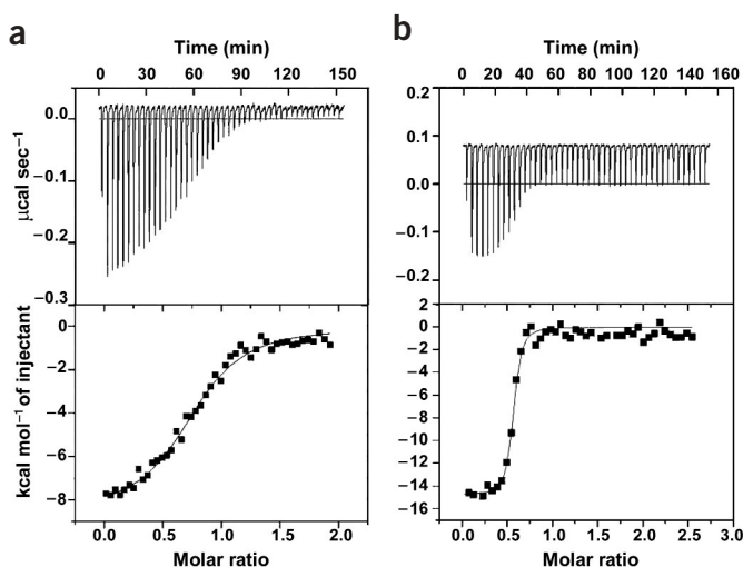
Figure 2 Binding of Cks1 to Cdk2 (left) and Cks1 to Skp1-Skp2 (right). Binding was measured by ITC.
